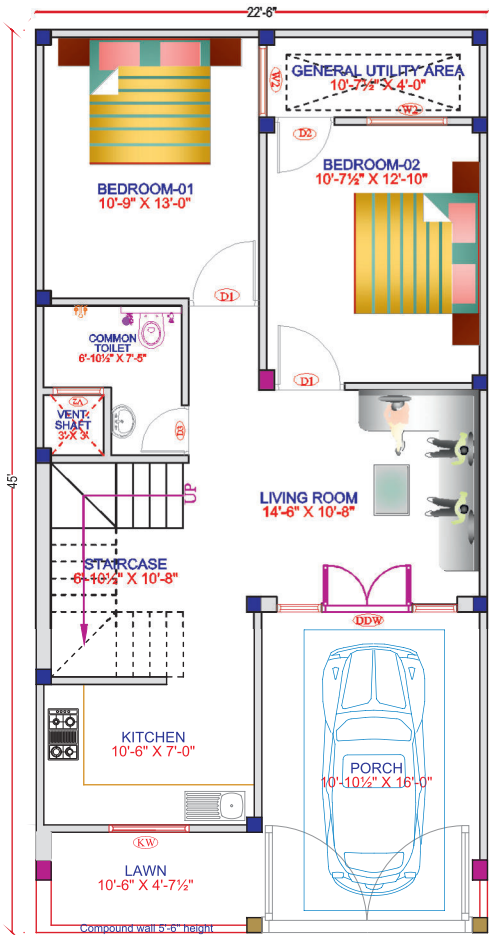
GROUND FLOOR KEY PLAN FOR DOOR WINDOW SCHEDULE
