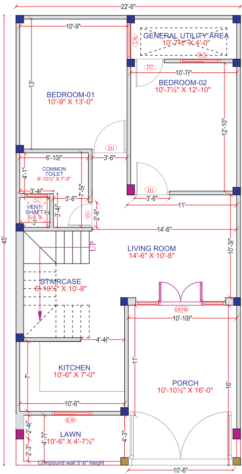
GROUND FLOOR WORKING PLAN
